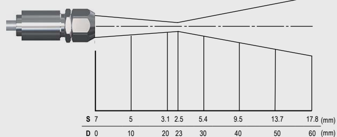
Optics CT LT CF, D:S = 2:1 (far field = 2.5:1)
